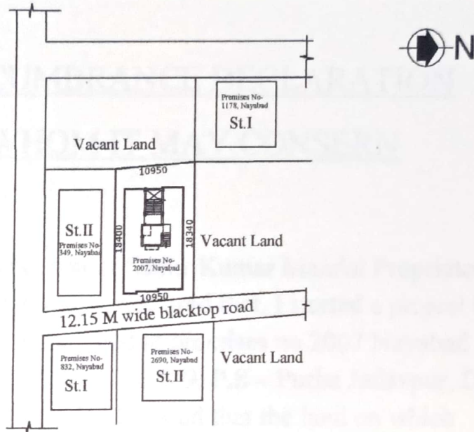
SITE PLAN
